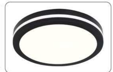
MSS-23 Ø380 x H45 LED 50W - IP65 3000K - 4000K - 6500K 1.220.000đ
