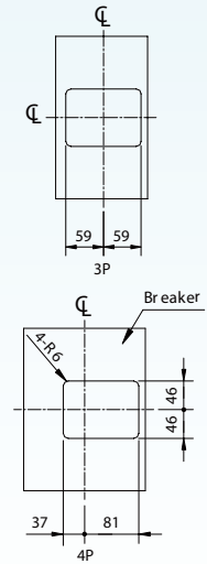
Panel cut
