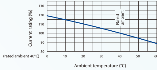
Compensation Curve
