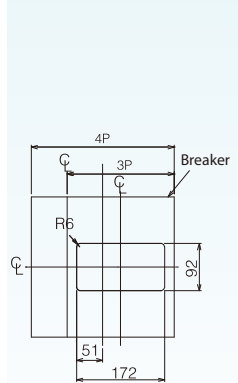
Panel cut
