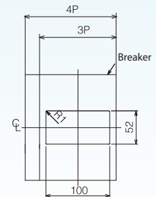
Panel cut
