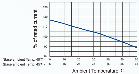
Compensation Curve
