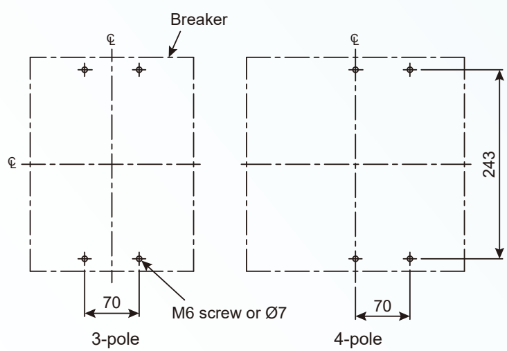
Bus drilling for direct connection
