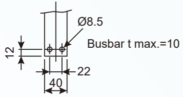
Bus drilling for direct connection
