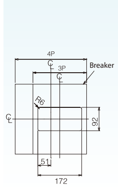
Panel cut
