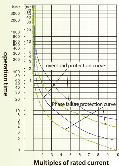
TH-P20ES TAPP tripping characteristic curve
