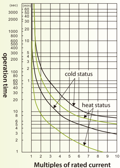
TH-P220ECT, TH-P400ECT, TH-P220TE, TH-P400TE 160A tripping characteristic curve
