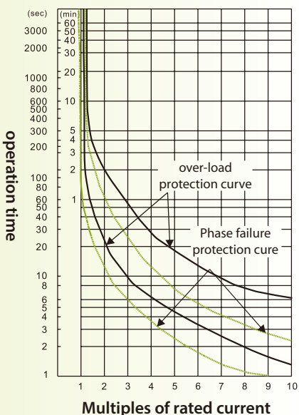
TH-P12ES PP tripping characteristic curve
