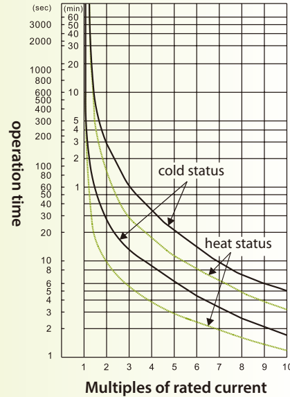
TH-P60ES TA tripping characteristic curve
