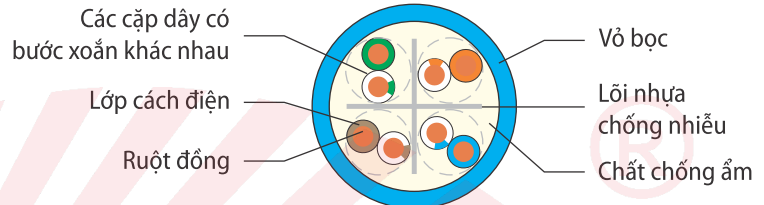
UTP/CAT6/SN/CA
