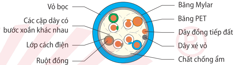
FTP/CAT5E/SN/CA
