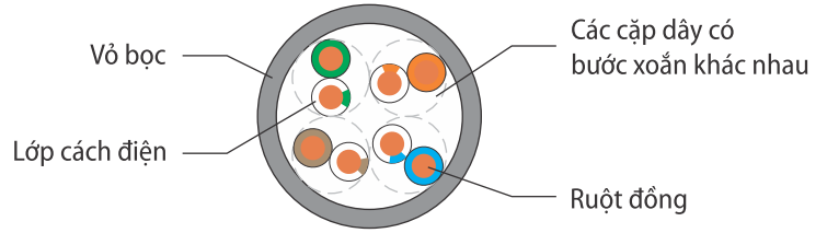
UTP/CAT5E/VL
